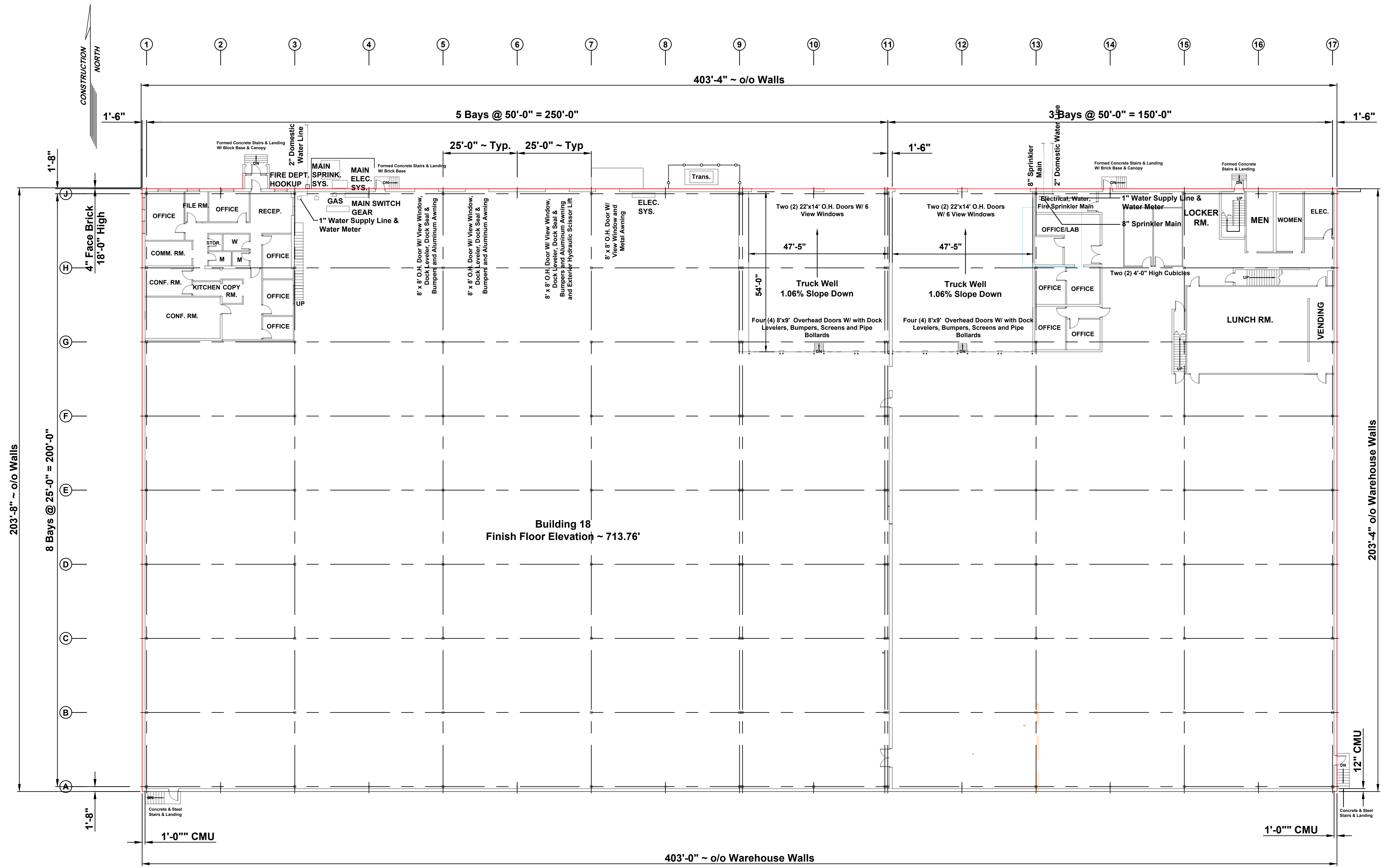
Building 18 / 18a Warehouse Floor Plan
